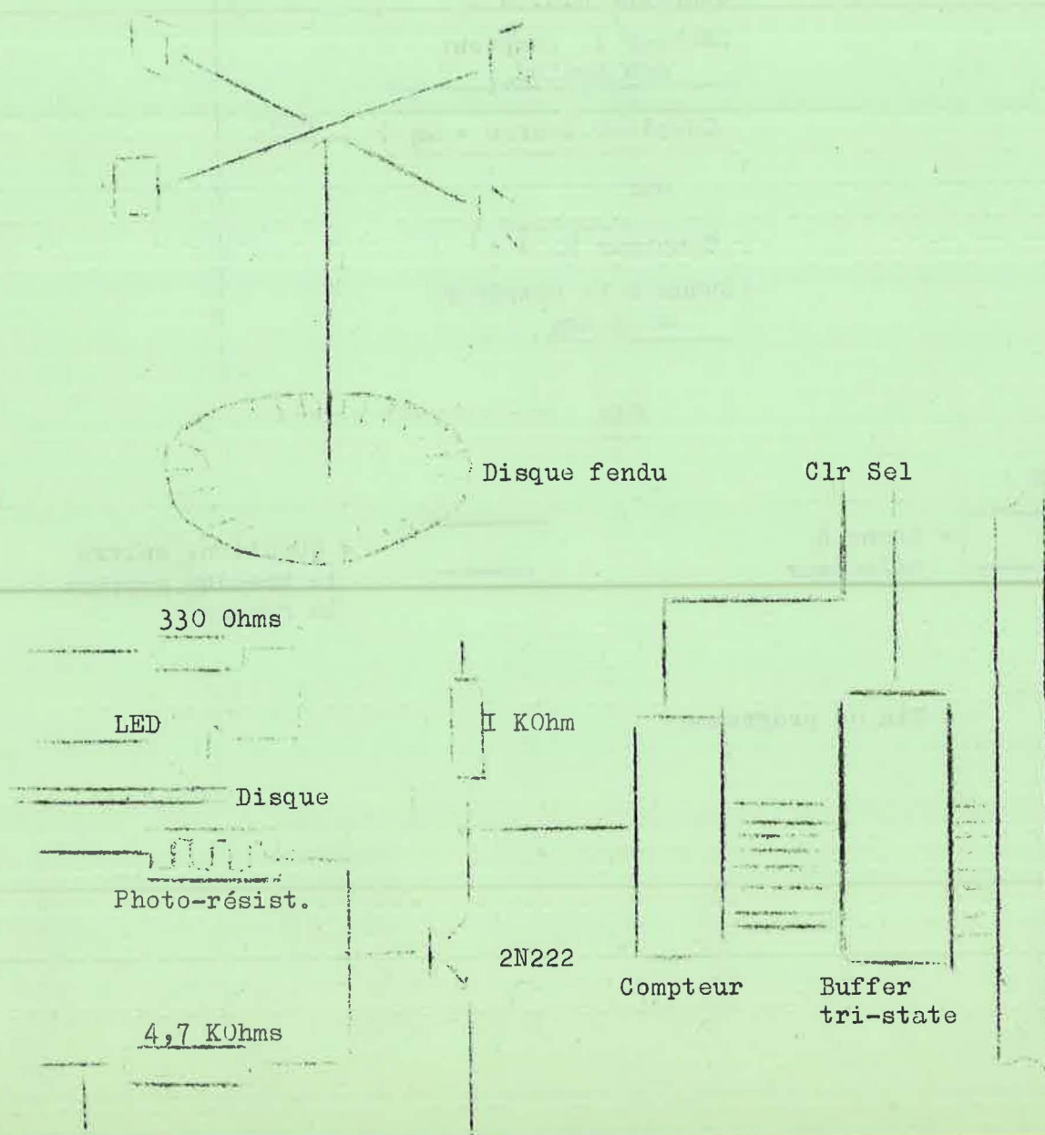
FIGURE 6 : ANEMOMETRE
